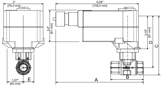
Actuator (V-FDV24) with 2-Way CVS
